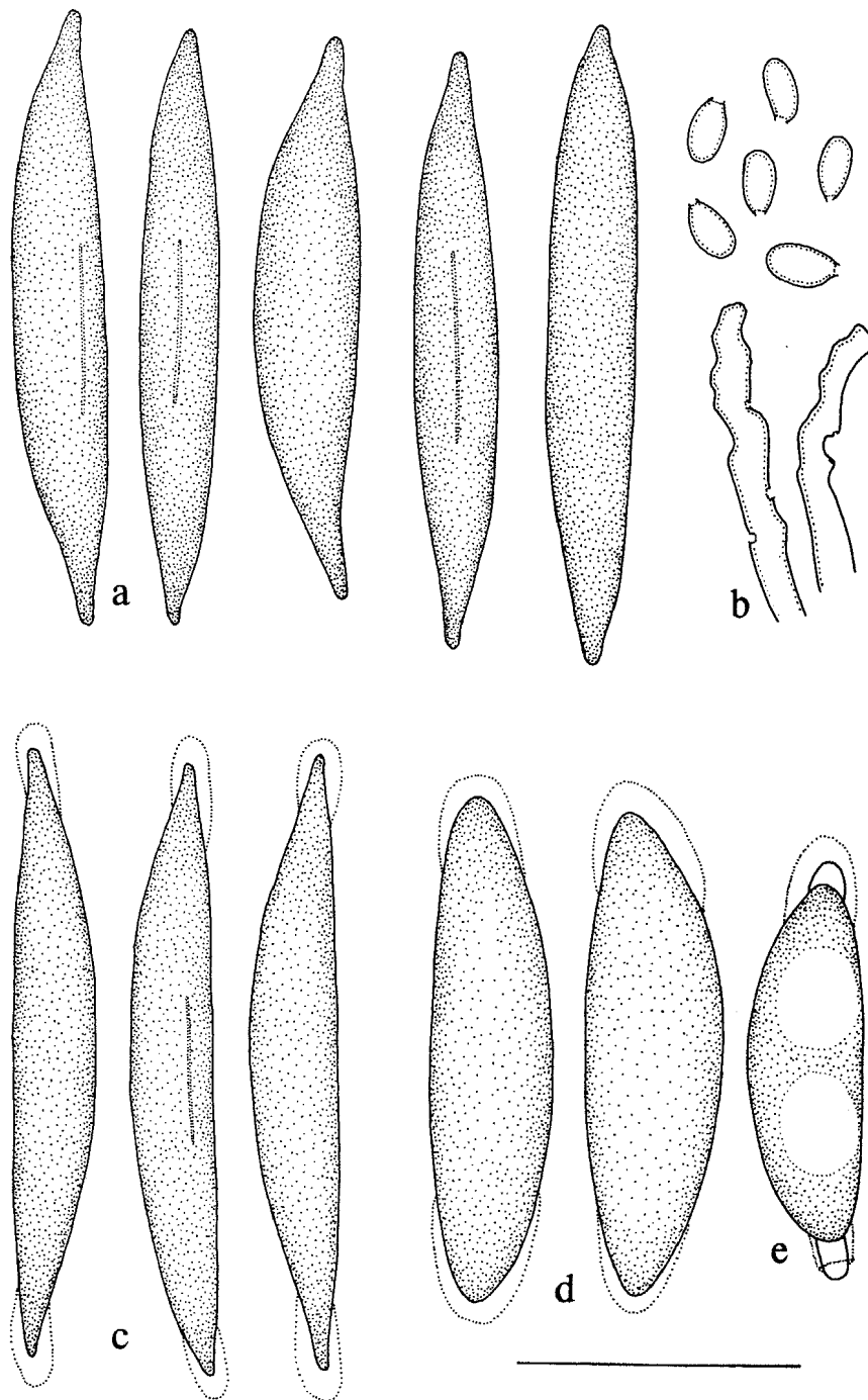
Fig. 2. Rosellinia necatrix (IMI 13328): a Ascospores. – b. Conidia and conidiophore tips. – Rosellinia bothrina (Holotype, K): c. Ascospores. – Rosellinia sp., “broad spore” (Ceylon 299, K): d. Ascospores. – Rosellinia aquila (IMI 204601): e. Ascospore. – bar = 20 \mu m.
