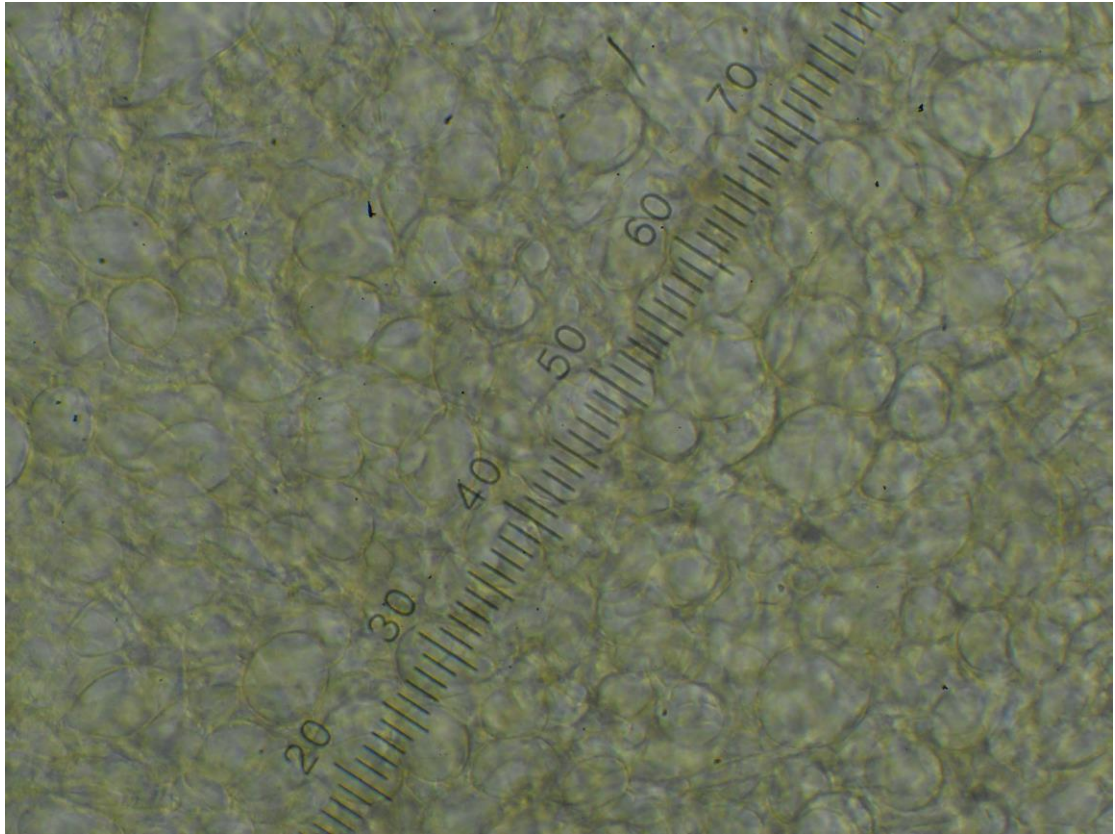
Asci dimensions 288-320 x 13-15,5 \mu\text{m}
